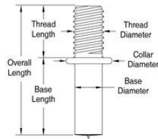
0.280 X 13mm with M8-1.25 X 16mm Extension, Stainless Steel, Capacitor Discharge Collar Stud Weld Stud
